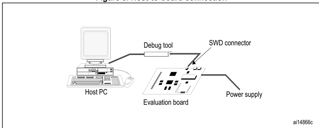
Figure 8. Host-to-board connection
