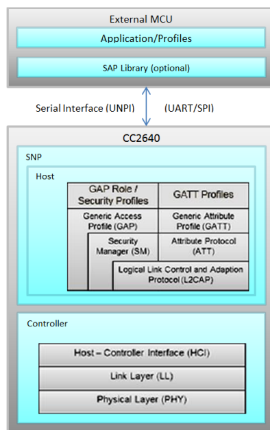
Figure 2-3. Simple Network Processor Configuration
