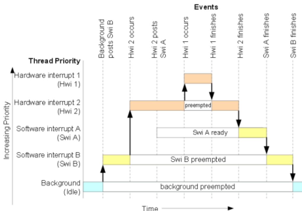
Figure 3-5. Preemption Scenario
