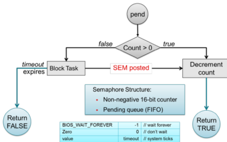
Figure 3-2. Semaphore Functionality
